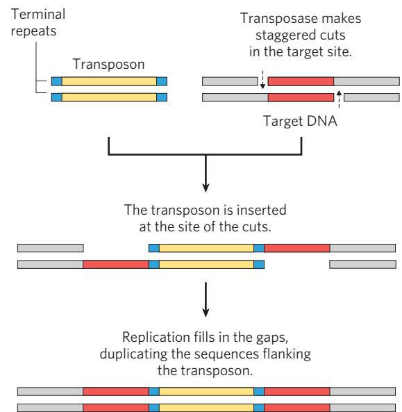
FIGURE 25–40 Duplication of the DNA sequence at a target site when a transposon is inserted. The sequences that are duplicated following transposon insertion are shown in red. These sequences are generally only a few base pairs long, so their size relative to that of a typical transposon is greatly exaggerated in this drawing.
