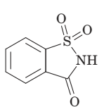
Saccharin MRS = 161 \Delta G^\circ = -9.7 kcal/mol
