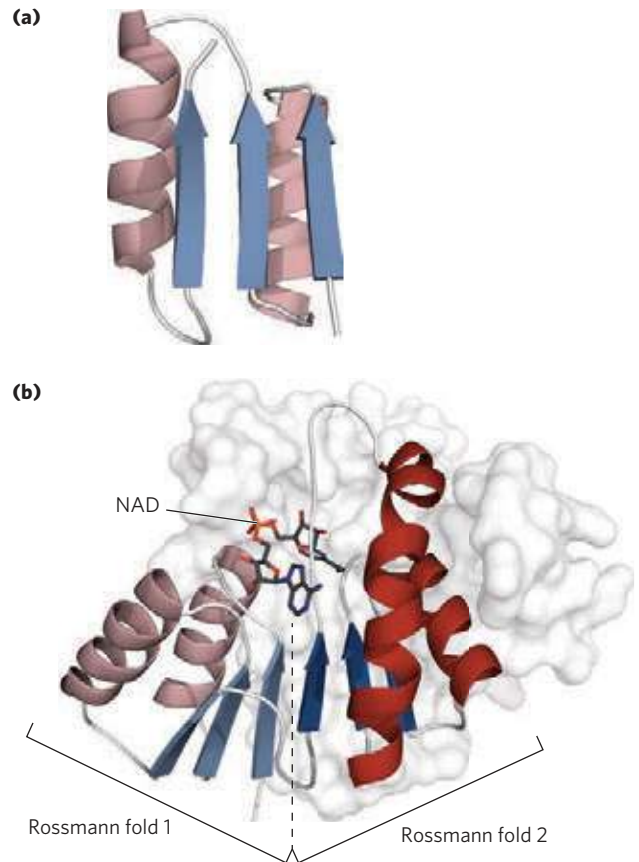
FIGURE 13–25 The Rossmann fold. This structural motif is found in the NAD-binding site of many dehydrogenases. (a) It consists of a pair of structurally similar motifs (only one of which is shown here), each having three parallel \beta sheets and two \alpha helices ( \beta - \alpha - \beta - \alpha - \beta ). (b) The nucleotide-binding domain of the enzyme lactate dehydrogenase (derived from PDB ID 3LDH) with NAD (ball-and-stick structure) bound in an extended conformation through hydrogen bonds and salt bridges to the paired \beta - \alpha - \beta - \alpha - \beta motifs of the Rossmann fold (shades of red and blue).
