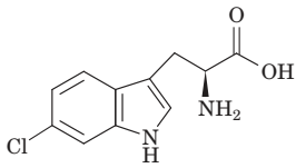
6-Chloro-D-tryptophan MRS = 906 \Delta G^\circ = -10.7 kcal/mol
