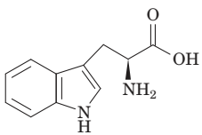
D-Tryptophan MRS = 21 \Delta G^\circ = -8.5 kcal/mol
