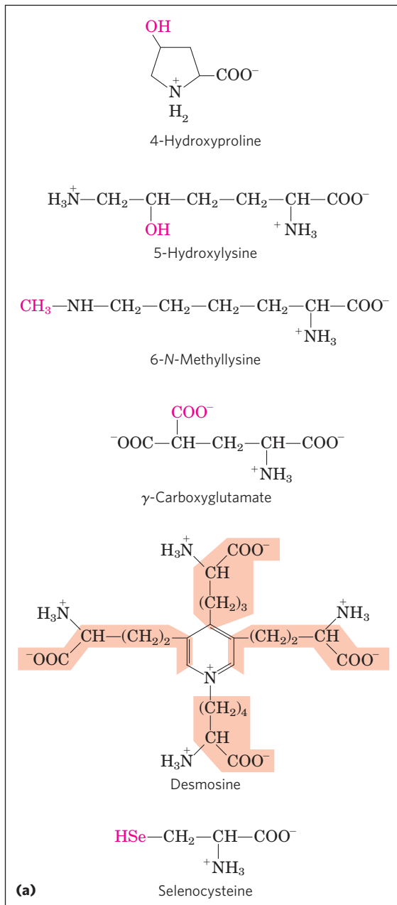
FIGURE 3-8 Uncommon amino acids. (a) Some uncommon amino acids found in proteins. All are derived from common amino acids. Extra functional groups by modification reactions are shown in red. Desmosine is formed from four Lys residues (the carbon backbones are shaded in light red). Note the use of either numbers or Greek letters in the names of these structures to identify the altered carbon atoms. (b) Reversible amino acid modifications involved in regulation of protein activity. Phosphorylation is the most common type of regulatory modification. (c) Ornithine and citrulline, which are not found in proteins, are intermediates in the biosynthesis of arginine and in the urea cycle.
