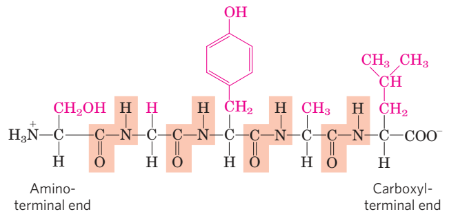
FIGURE 3-14 The pentapeptide serylglycyltyrosylalanylleucine, Ser-Gly-Tyr-Ala-Leu, or SGYAL. Peptides are named beginning with the amino-terminal residue, which by convention is placed at the left. The peptide bonds are shaded in light red; the R groups are in red.
