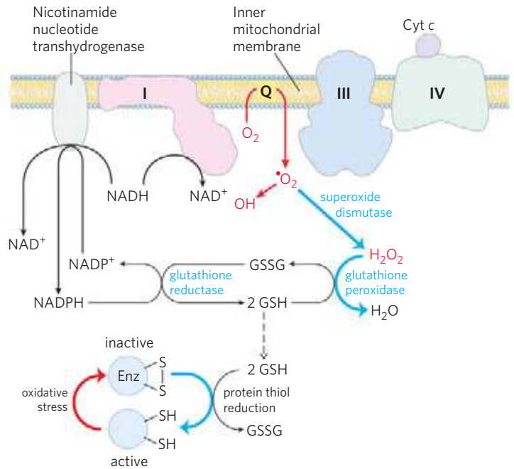
FIGURE 19–18 ROS formation in mitochondria and mitochondrial defenses. When the rate of electron entry into the respiratory chain and the rate of electron transfer through the chain are mismatched, superoxide radical ( \cdot\text{O}_2^- ) production increases at Complexes I and III as the partially reduced ubiquinone radical ( \cdot\text{Q}^- ) donates an electron to \text{O}_2 . Superoxide acts on aconitase, a 4Fe-4S protein, to release \text{Fe}^{2+} . In the presence of \text{Fe}^{2+} , the Fenton reaction leads to formation of the highly reactive hydroxyl free radical ( \cdot\text{OH} ). The reactions shown in blue defend the cell against the damaging effects of superoxide. Reduced glutathione (GSH; see Fig. 22–29) donates electrons for the reduction of \text{H}_2\text{O}_2 and of the oxidized Cys residues ( -\text{S}-\text{S}- ) of enzymes and other proteins, and GSH is regenerated from the oxidized form (GSSG) by reduction with NADPH.
