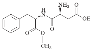
Aspartame MRS = 172 \Delta G^\circ = -9.7 kcal/mol
