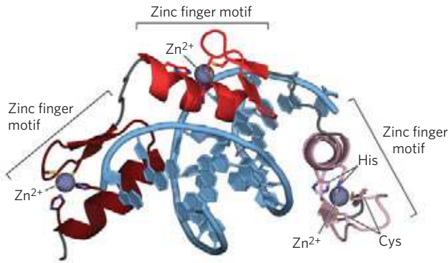
FIGURE 28-12 Zinc fingers. (PDB ID 1ZAA) Three zinc fingers (shades of red) of the regulatory protein Zif268, complexed with DNA (blue). Each \text{Zn}^{2+} coordinates with two His and two Cys residues.
