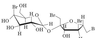
Tetrabromosucrose MRS = 13,012 \Delta G^\circ = -12.2 kcal/mol
