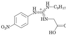
Sucronic acid MRS = 200,000 \Delta G^\circ = -13.8 kcal/mol
