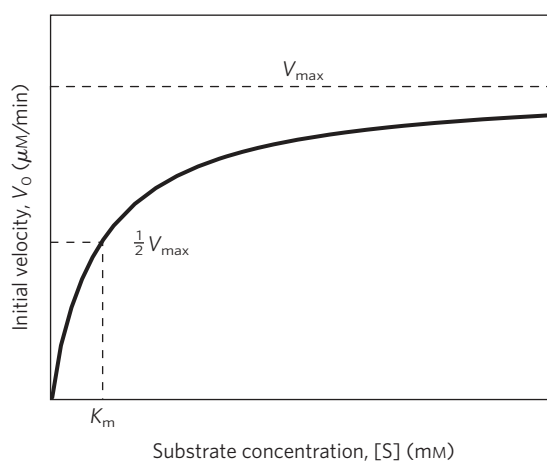
FIGURE 6-11 Effect of substrate concentration on the initial velocity of an enzyme-catalyzed reaction. The maximum velocity, V_{\max} , is extrapolated from the plot, because V_0 approaches but never quite reaches V_{\max} . The substrate concentration at which V_0 is half maximal is K_m , the Michaelis constant. The concentration of enzyme in an experiment such as this is generally so low that [S] \gg [E] even when [S] is described as low or relatively low. The units shown are typical for enzyme-catalyzed reactions and are given only to help illustrate the meaning of V_0 and [S] . (Note that the curve describes part of a rectangular hyperbola, with one asymptote at V_{\max} . If the curve were continued below [S] = 0 , it would approach a vertical asymptote at [S] = -K_m .)
