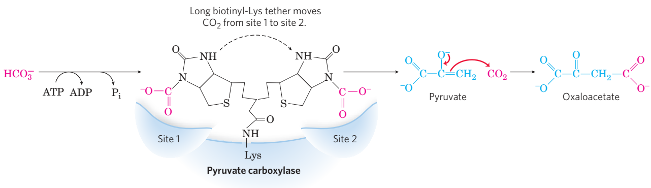
FIGURE 14-19 Role of biotin in the pyruvate carboxylase reaction. The cofactor biotin is covalently attached to the enzyme through an amide linkage to the ε-amino group of a Lys residue, forming a biotinyl-enzyme. The reaction occurs in two phases, which occur at two different sites in the enzyme. At catalytic site 1, bicarbonate ion is converted to CO 2 at the expense of ATP. Then CO 2 reacts with biotin, forming carboxybiotinyl-enzyme. The long arm composed of biotin and the Lys side chain to which it is attached then carry the CO 2 of carboxybiotinyl-
