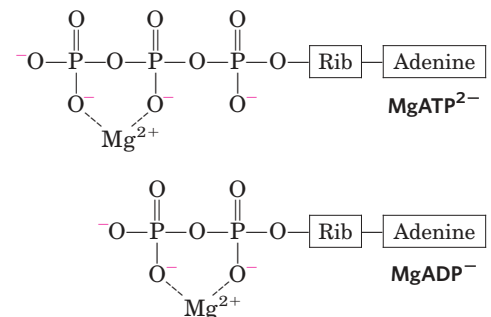
FIGURE 13–12 \text{Mg}^{2+} and ATP. Formation of \text{Mg}^{2+} complexes partially shields the negative charges and influences the conformation of the phosphate groups in nucleotides such as ATP and ADP.
