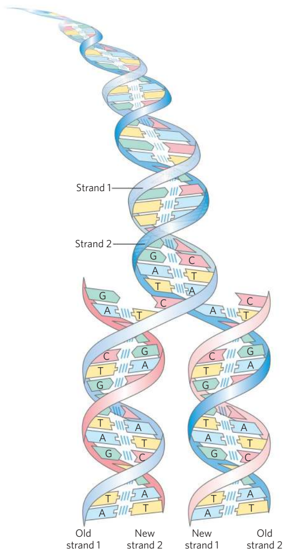
FIGURE 1-31 Complementarity between the two strands of DNA.
